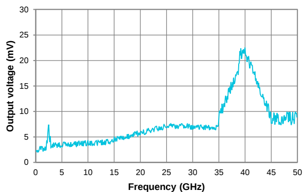
High power frequency response
